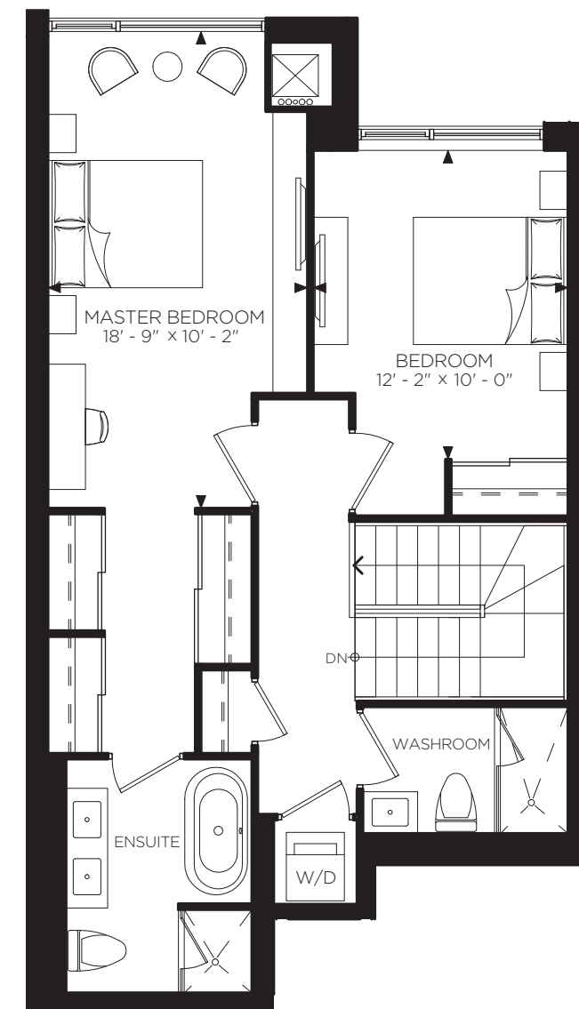
LEVEL 8
